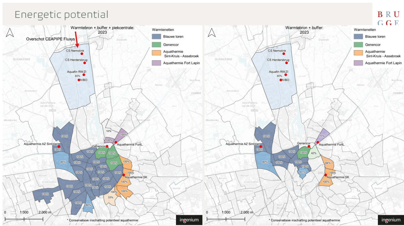
Energy potential based on heat sources, City of Bruges
